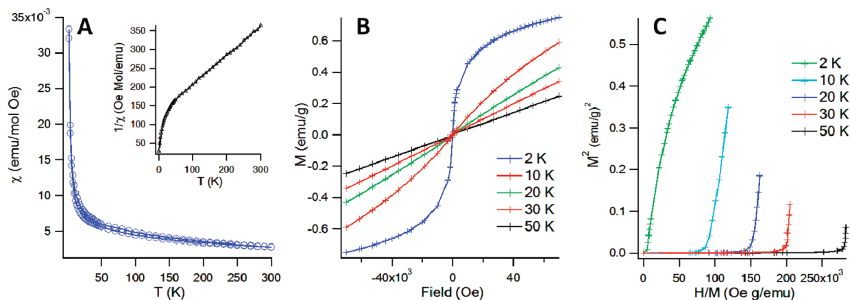
Figure 6. (A) Temperature-dependent ZFC and FC (200 Oe) susceptibility data. The insert is the C–W law plot showing negative C–W temperature ( -125 K). (B) Field-dependent magnetization ( M ) plots at 2, 10, 20, 30, 50 K, and (C) Arrott plots ( M^2 vs H/M ) for the 2.5% \text{Zn}_{1-x}\text{Cr}_x\text{Se} QDs.
