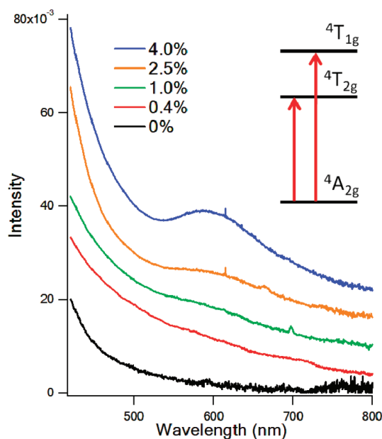
Figure 3. Absorption spectra (298 K) in concentrated toluene solution for 0, 0.4, 1.0, 2.5, and 4.0 Zn 1-x Cr x Se QDs. Inset shows the allowed crystal field transitions of Cr(III) ion in an O h crystal field.
