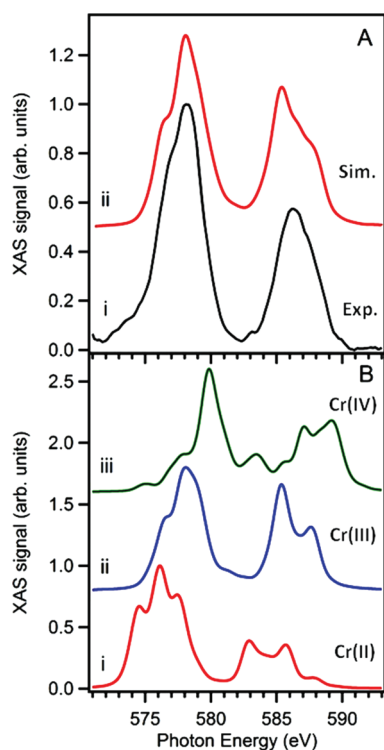
Figure 2. Cr L 2,3 edge X-ray absorption spectra. (A) (i) 2.5% Zn 1-x Cr x Se QDs and (ii) simulated tetragonally distorted O h crystal field (2.07 eV) for Cr(III). (B) XANES simulation of Cr ions in a perfect O h field (10 D q = 2.07 eV): (i) Cr(II), (ii) Cr(III), and (iii) Cr(IV).
