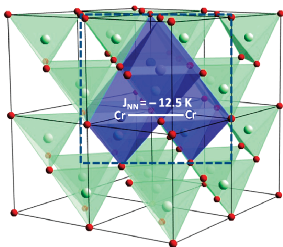
Figure 5. Illustration of the \text{ZnCr}_2\text{Se}_4 spinel structure composed of 4 \text{CrSe}_6 O_h units embedded in the \text{ZnSe} zinc-blende lattice. The \text{Cr(III)} ions (blue balls) occupy O_h sites, and \text{Zn(II)} ions (green balls) occupy T_d sites.
